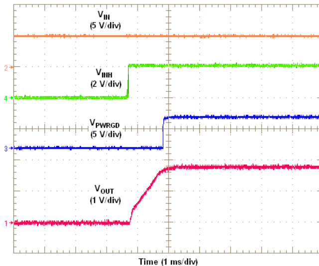
Figure 24. Inhibit Turn-On
